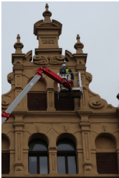
Rotatable jib (180 °) and platform (2x 90 °)
